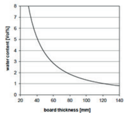
Figure 3: Influence of board thickness on water absorption by diffusion (EN 12088) (fusion >95 %; 30 kg/m³)
